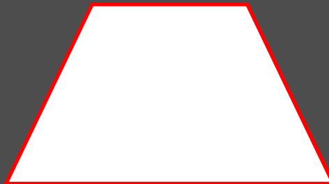
Trapez
